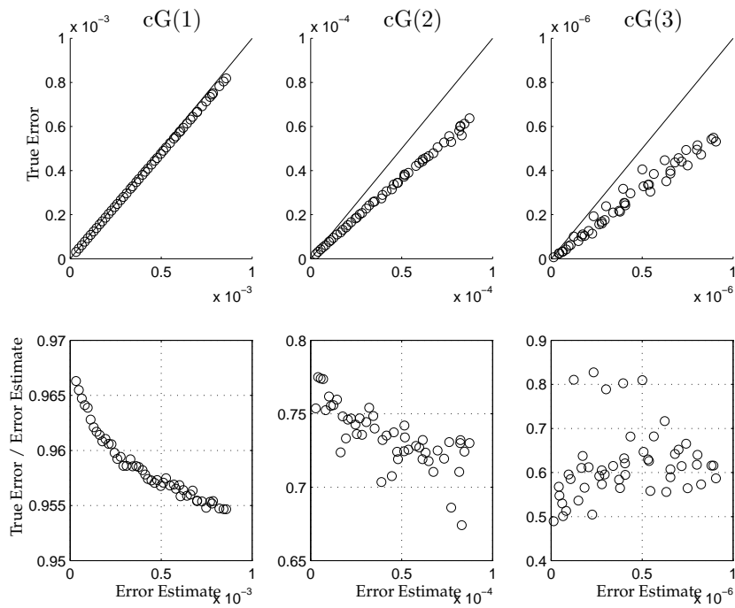
Figure 4.10: True error vs. error estimate for multi-adaptive cG(1), cG(2) and cG(3) respectively. Solid lines indicate the ideal maximum size of the true error.
