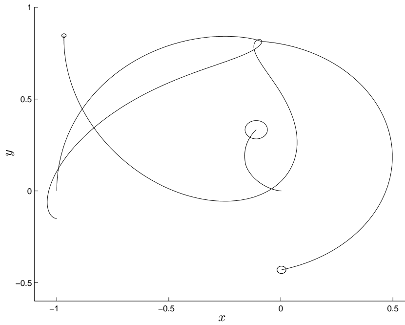
Figure 4.5: Orbits for the three planets. The circles drawn represent the planets at time t = T .
