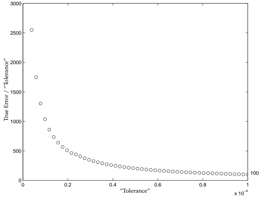
Figure 4.11: True error / tolerance vs. tolerance for MATLAB:s ODE-solver ode45 ( ).
