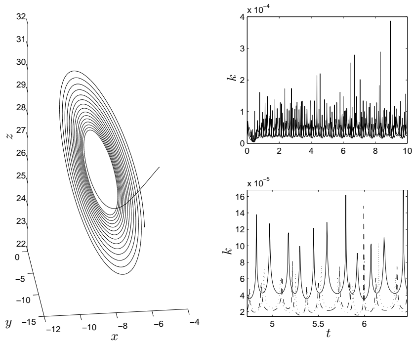
Figure 4.8: At the left is the solution of the Lorenz system, solved with the multadaptive cG(1) method at TOL = 2.5 \cdot 10^{-5} and with final time T = 10 . At the right are the timesteps used for the computation.
