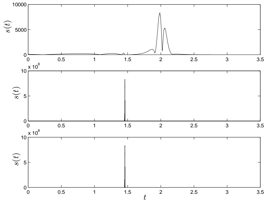
Figure 4.6: Stability functions for the x -components of the three planets.
