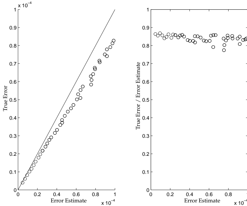
Figure 4.12: True error vs. error estimate for the multi-adaptive cG(1)-method. The solid lines indicate the ideal maximum size of the true error.
