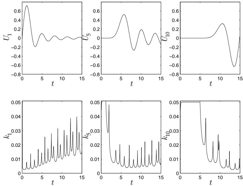
Figure 4.4: Solutions for components 1,5 and 10 of a system consisting of 10 masses and 11 springs, together with their respective timesteps, solved at TOL = 5 \cdot 10^{-4} with the multi-adaptive cG(1) method.
