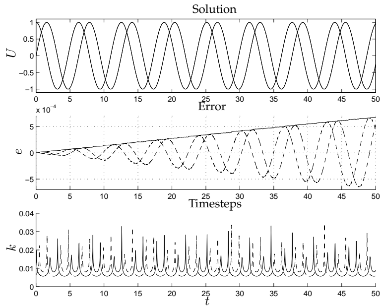
Figure 4.1: The solution of the simple harmonic oscillator problem, the errors and the timesteps respectively.
