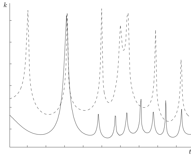
Figure 1.1: These are the actual timesteps used for an example computation on a simple two-dimensional system.
