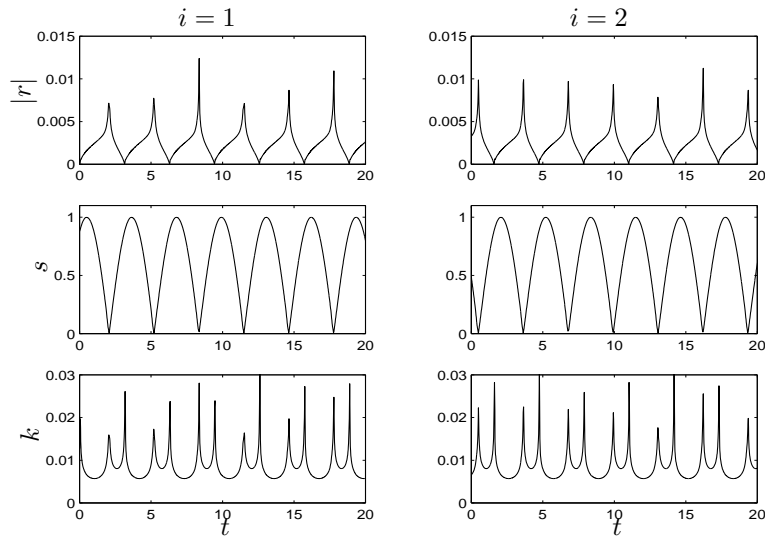
Figure 4.2: Residuals, stability functions and timesteps for the two components of the harmonic oscillator problem, shown for the interval (0, 20) .
