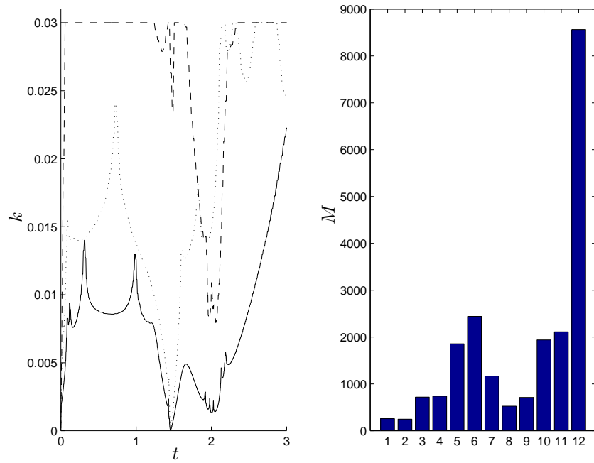
Figure 4.7: Timesteps (left) and the number of timesteps (right) for the 12 different components of the three-body problem.
