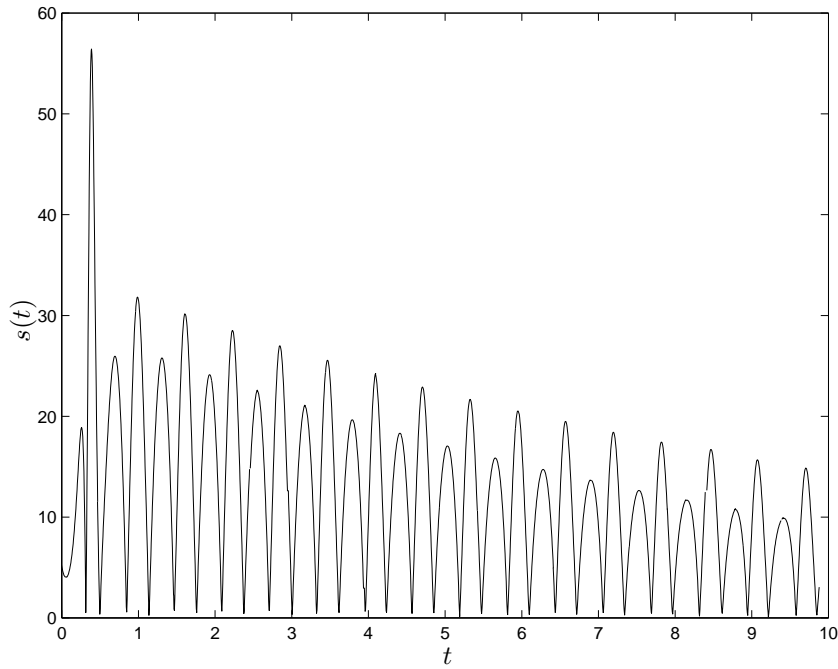
Figure 4.9: The figure shows the stability function s = s(t) for the y component of the Lorenz system. The other two components are similar to this one.
